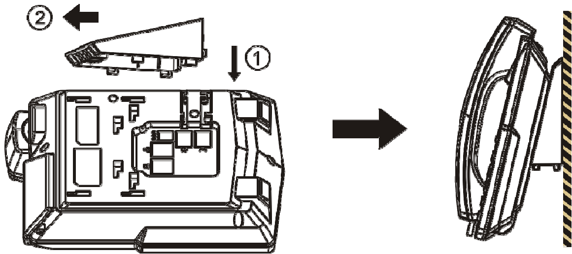
Figure 2 - Wall-mount Installation
