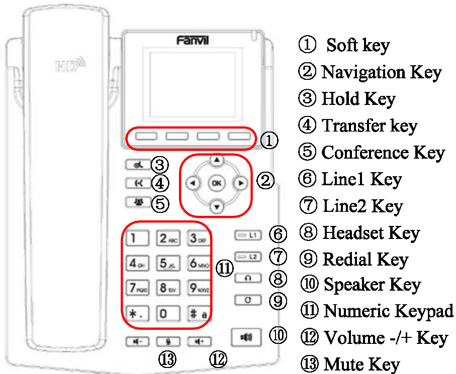
Figure 4 - Keypad
